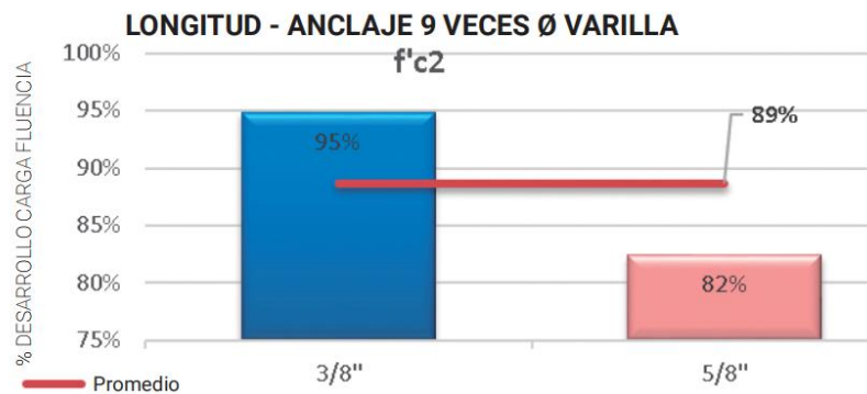
Figure 5. Anchorage length nine times the diameter, average strength. Source: own elaboration.
