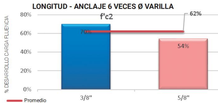
Figure 4. Anchor length six times the diameter, average strength. Source: own elaboration.
