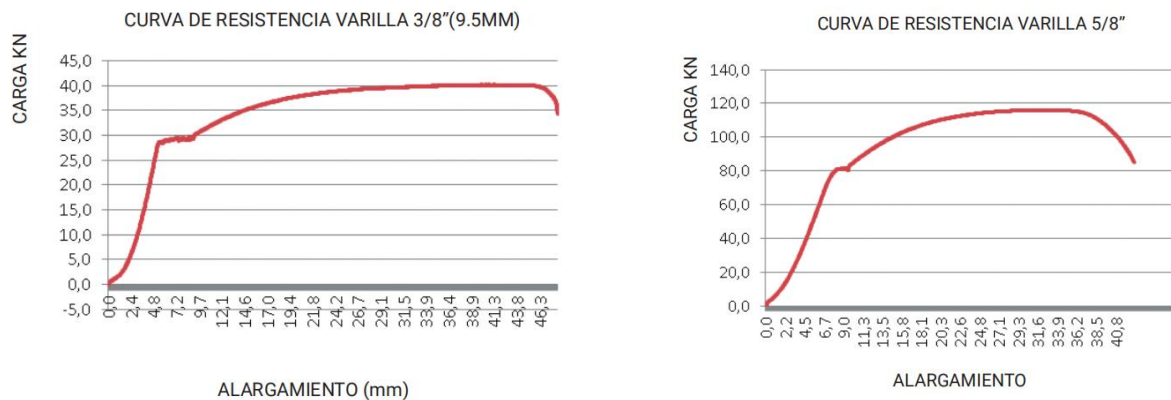
Figure 3. Tensile strength curves 3/8" (9.5 mm) and 5/8" (15.9 mm). Source: own elaboration.
