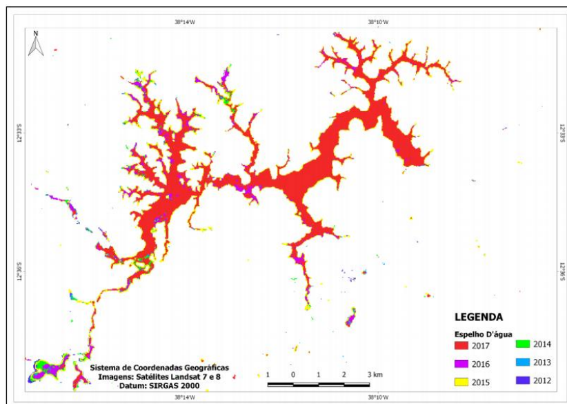
Figure 13. Dynamics of the water mirror of the Santa Helena reservoir, Bahia Source: Research results, 2022.
