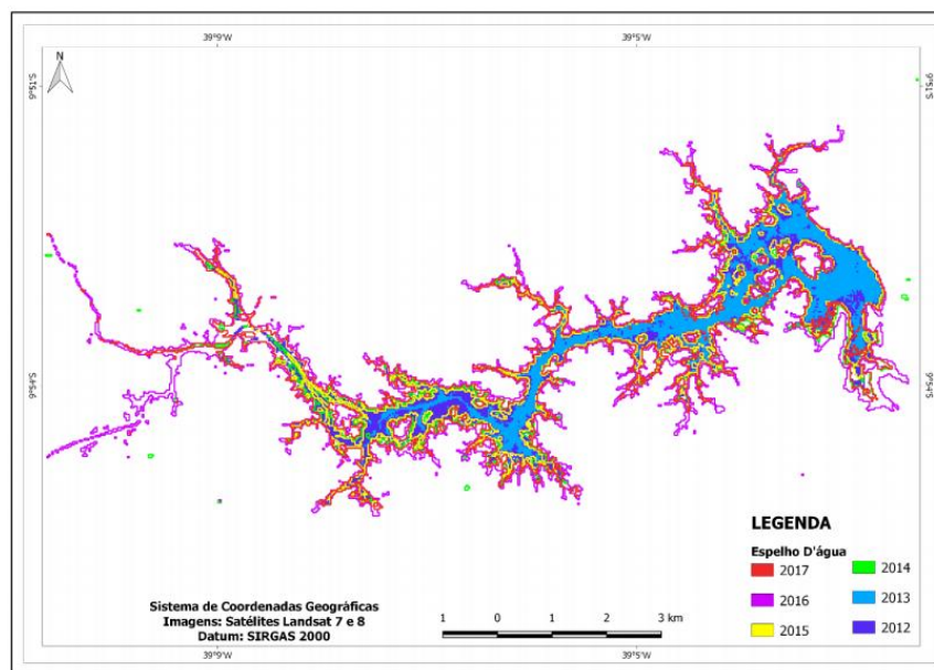
Figure 15. Dynamics of the water mirror of the Cocorobó reservoir, Bahia Source: Research results, 2022.
